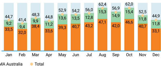
Volume Lapisan Tanah Penutup Bulanan Monthly Overburden Removal
